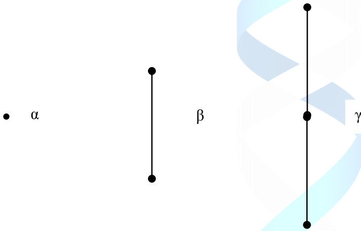
Figure 2. Bootstrap graphs after the collapse of towers
