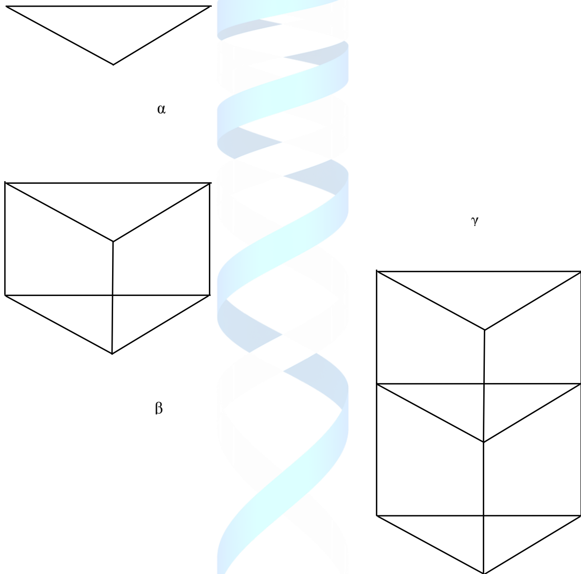
Figure 1. Bootstrap graphs
