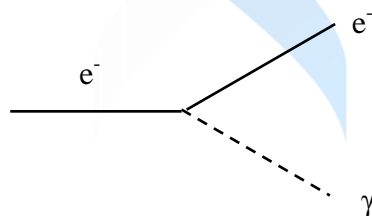
Figure 7. Example of crossed coupling. The time goes from left to right.
