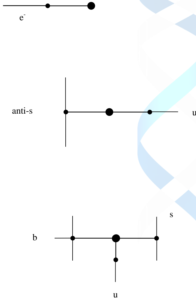
Figure 5. Glyphs of electron, meson u\bar{s} and baryon usb .
