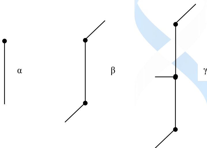
Figure 3. Bootstrap graphs after the collapse of towers and the application of external lines departing from vertices
