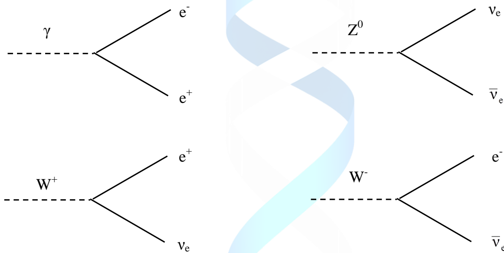
Figure 6. Examples of creation of particle-antiparticle pairs (top) and of pairs of particles having opposite values of weak isospin (down). The time is directed from the left to the right.
