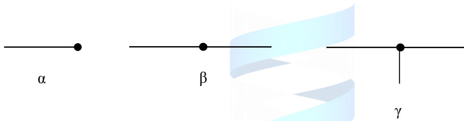
Figure 4. The same of Fig.2, after the collapse of vertices. Monadic, dyadic and triadic graphs of Peirce's theory are derived.
